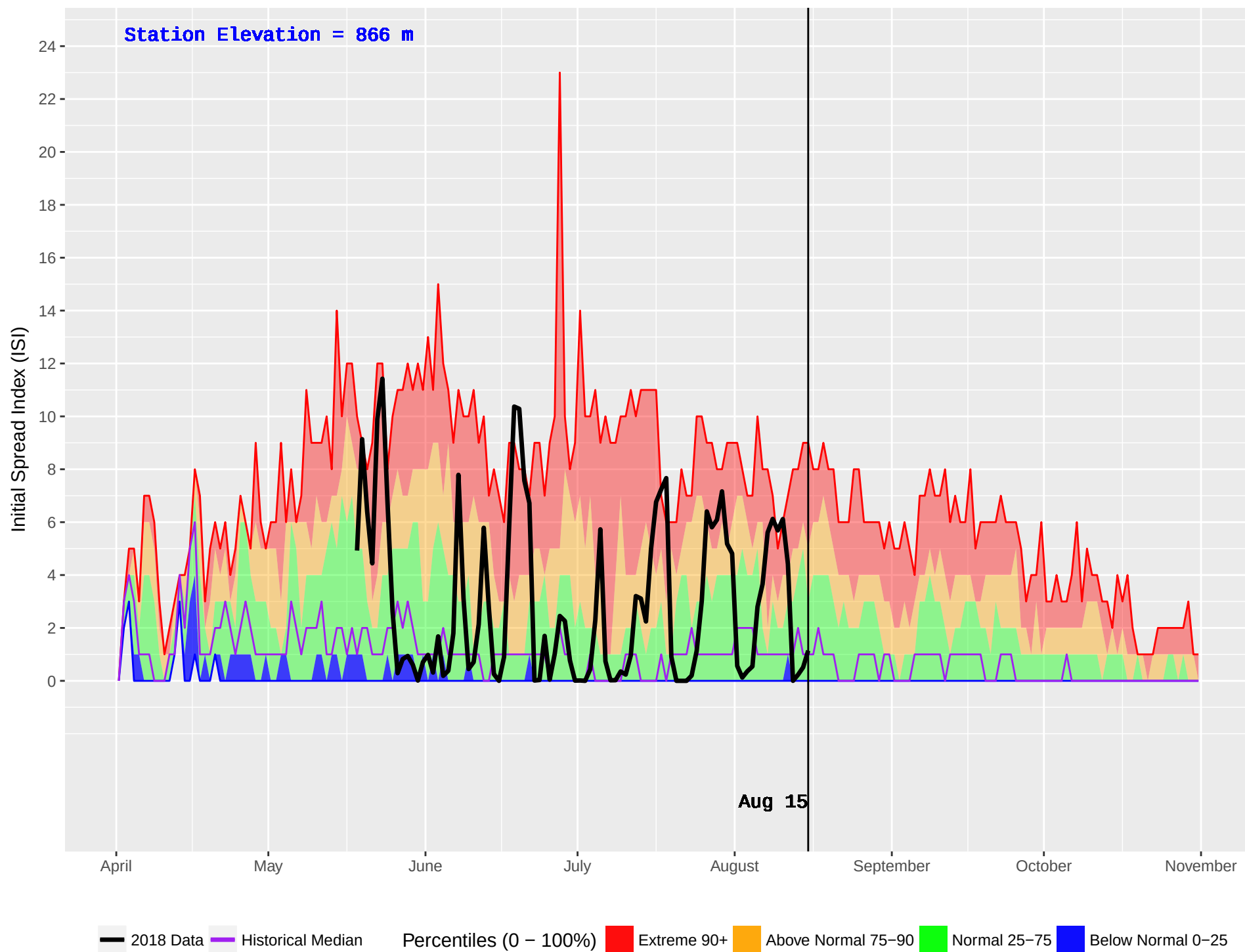
CATFISH (199) : Historical (1986–2016) and Current (2018) Daily Initial Spread Index (ISI)
