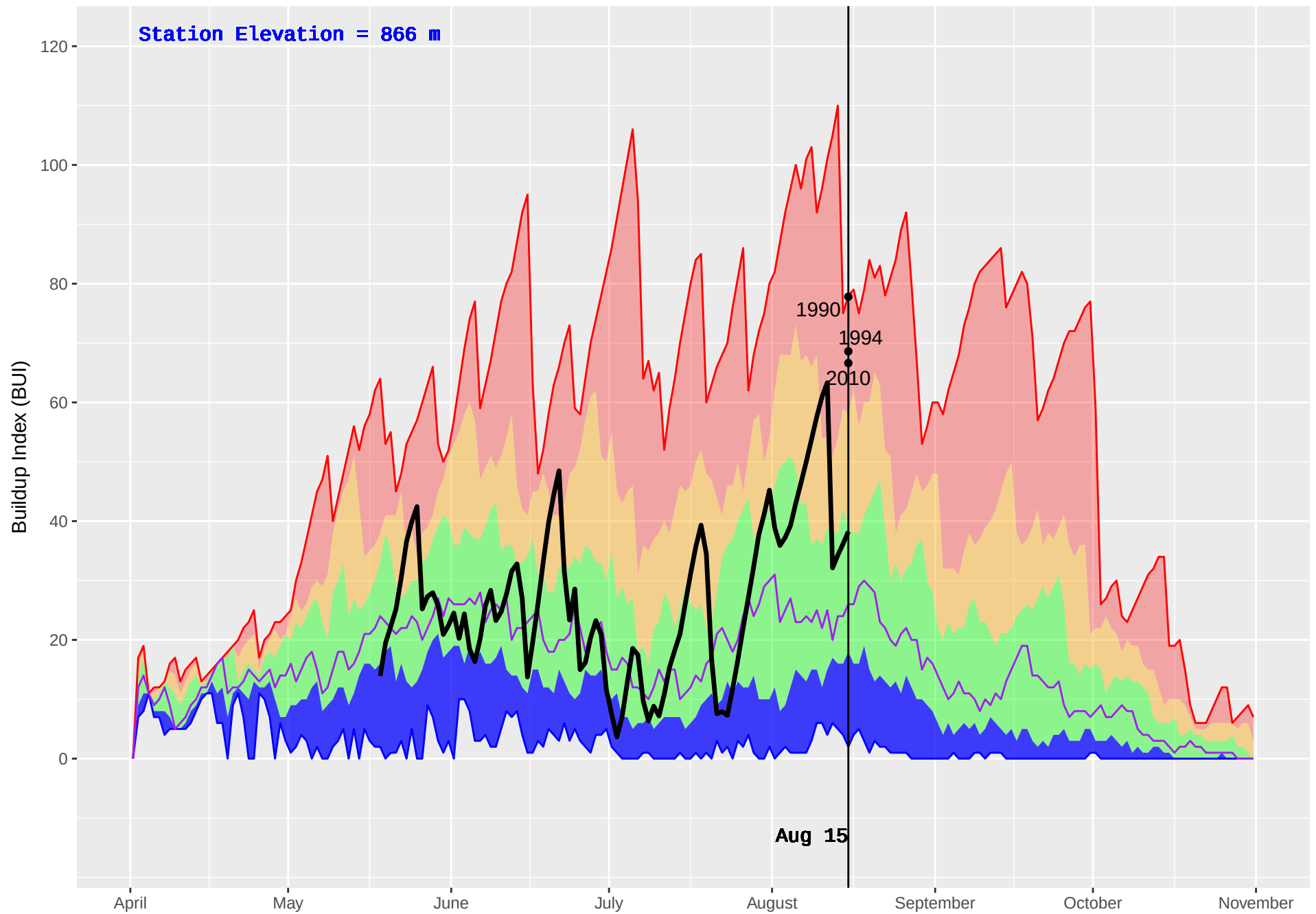
CATFISH (199) : Historical (1986–2016) and Current (2018) Daily Buildup Index (BUI)
