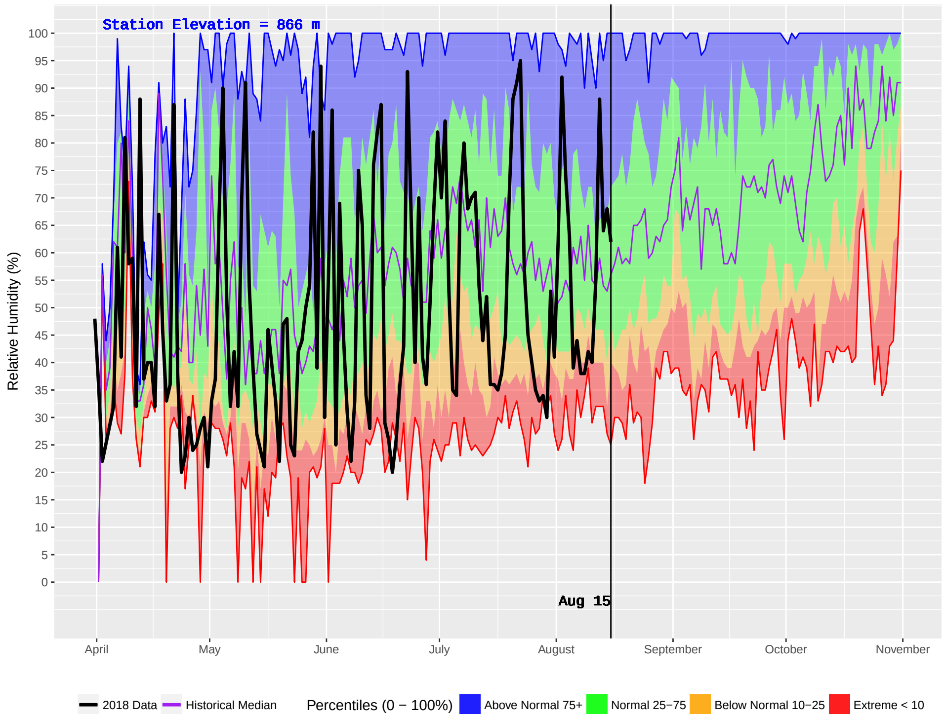
CATFISH (199) : Historical (1986–2016) and Current (2018) Daily Relative Humidity
