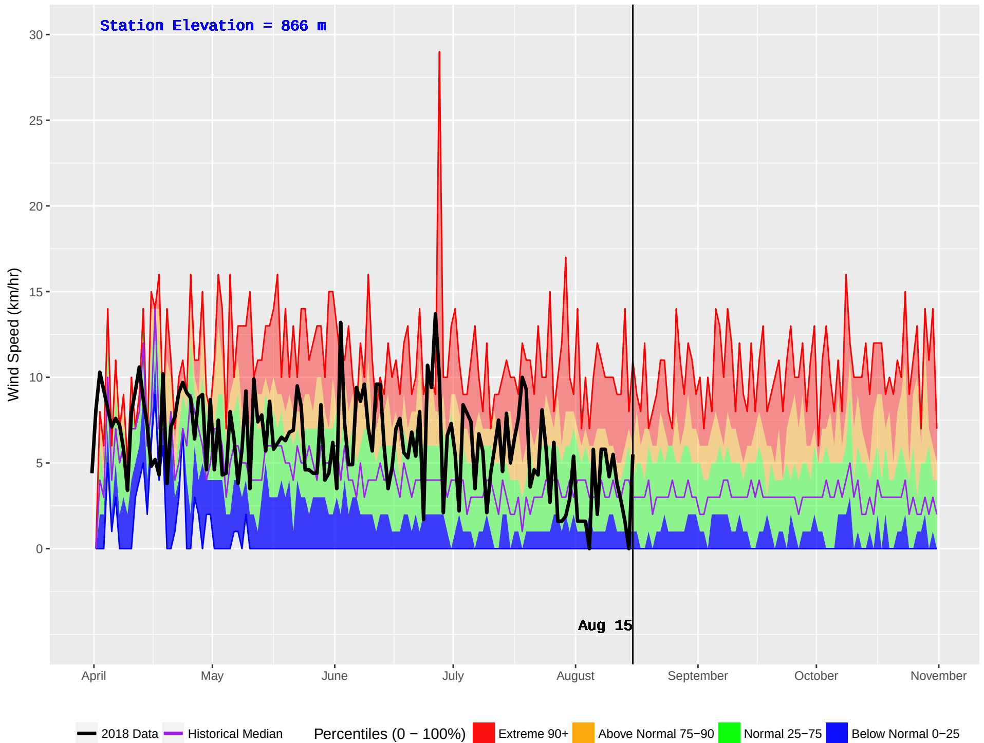
CATFISH (199) : Historical (1986–2016) and Current (2018) Daily Wind Speed
