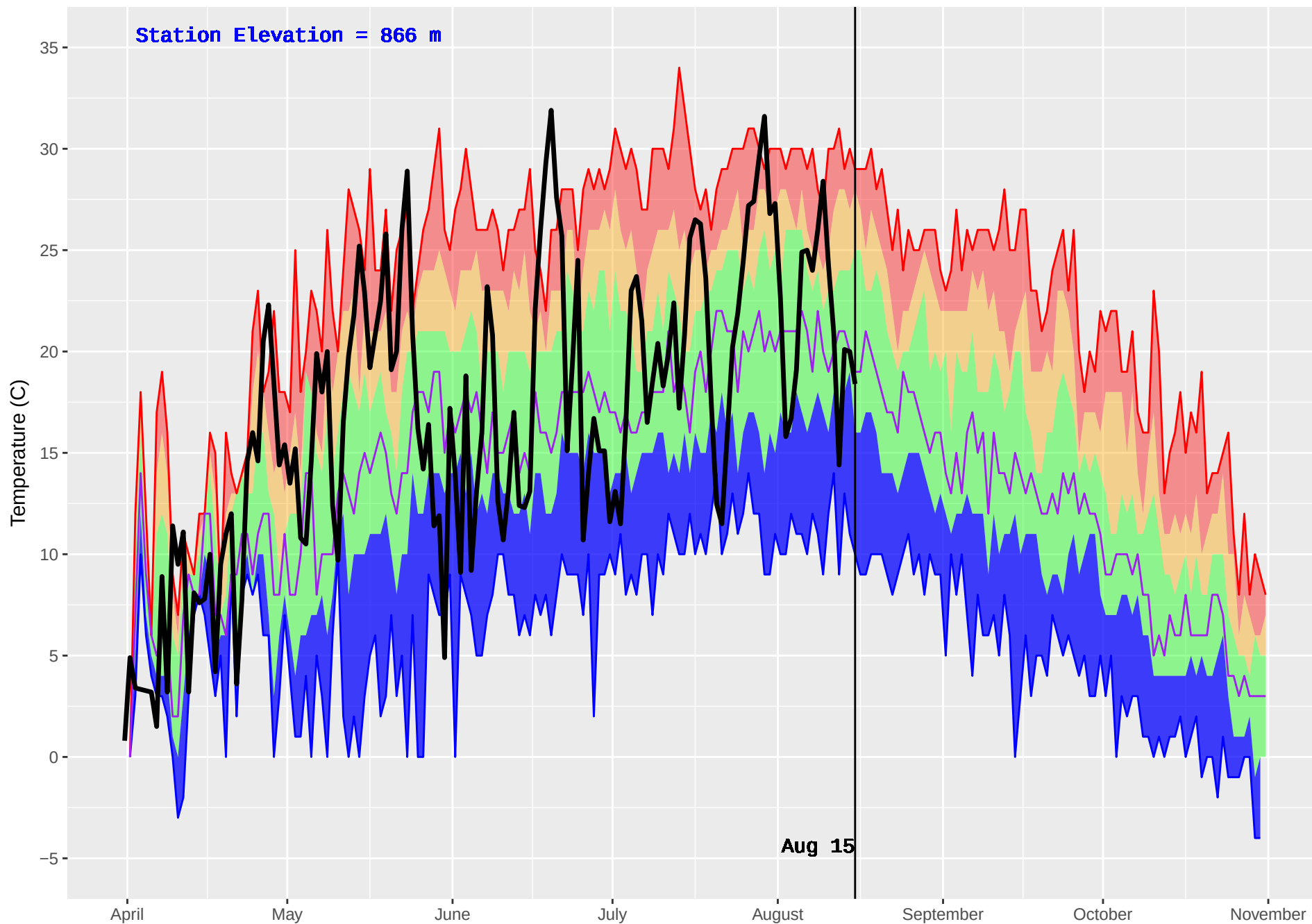
CATFISH (199) : Historical (1986–2016) and Current (2018) Daily Temperature
